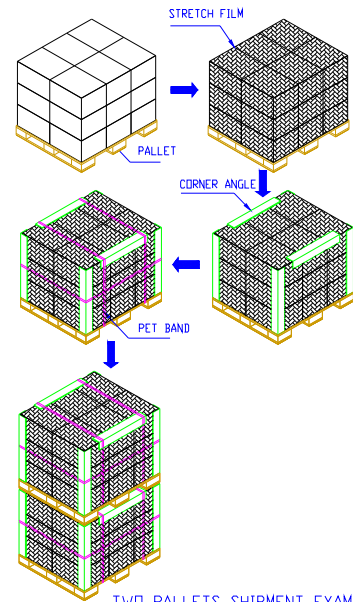
TWO PALLET SHIPMENT EXAMPLE SHIPPING BY SEA_HQ USED
