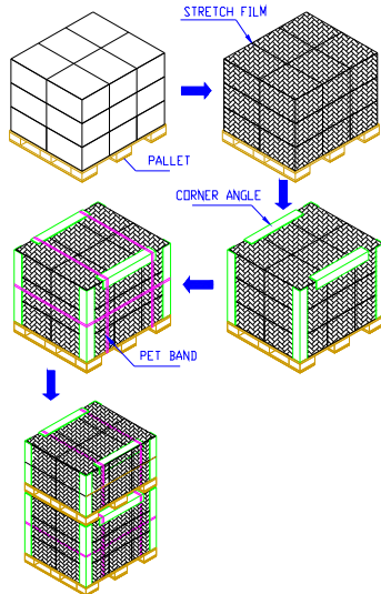
TWO PALLET SHIPMENT EXAMPLE SHIPPING BY SEA USED
