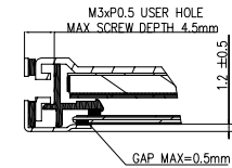
SECTION USER_HOLE-USER_HOLE SCALE 4:1
