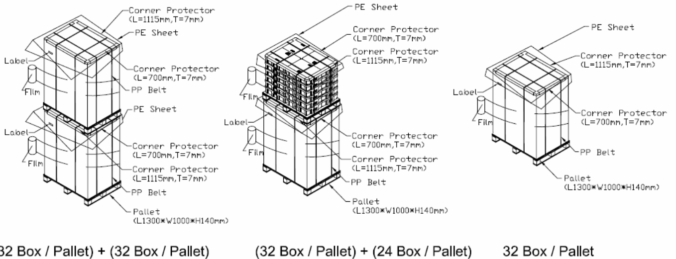
Figure.10-2 packing method
