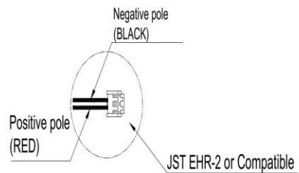
Connector View
