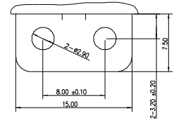
DETAIL D SCALE 5:1
