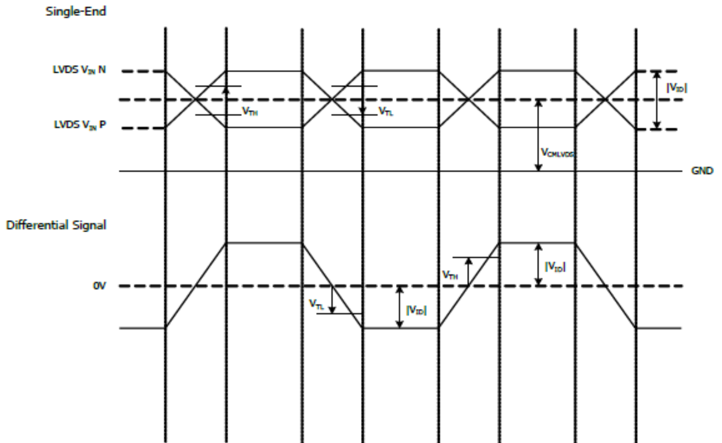
Figure 2: LVDS Waveform
