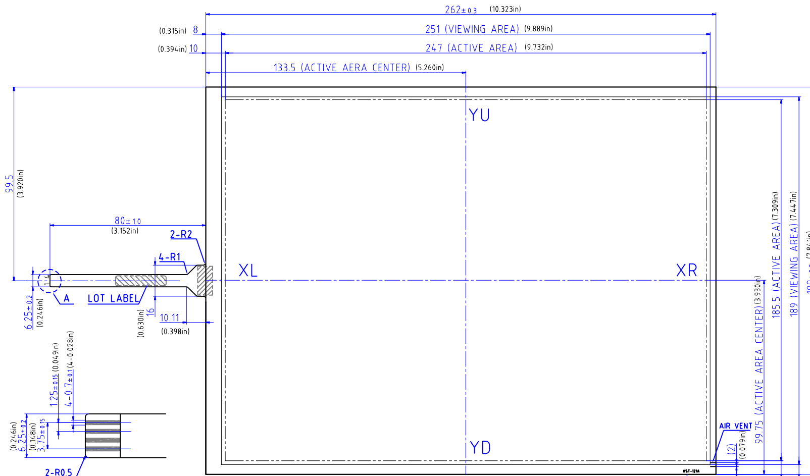
SECTION A
