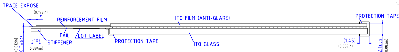
SECTION A
