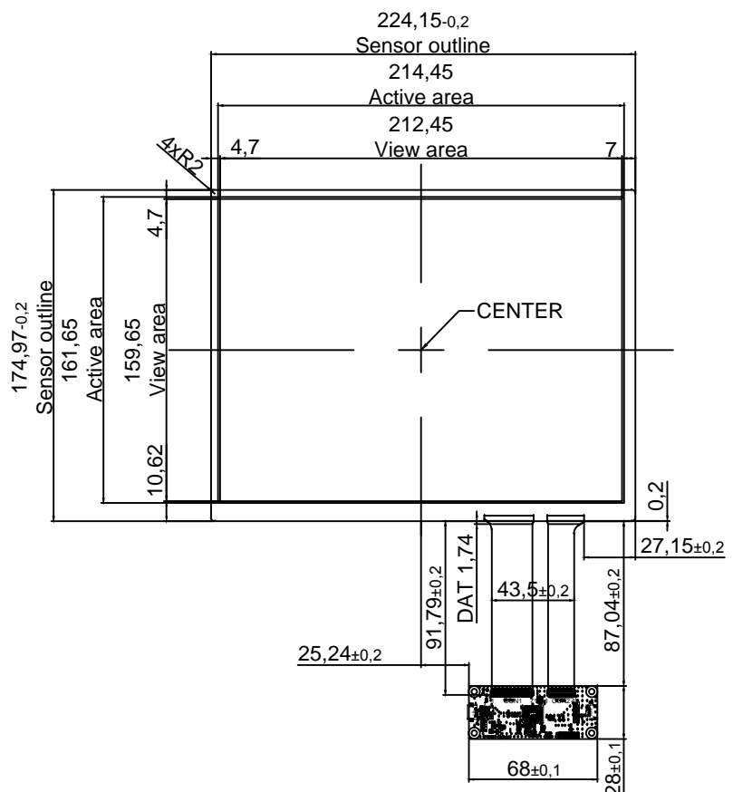
FRONT VIEW
