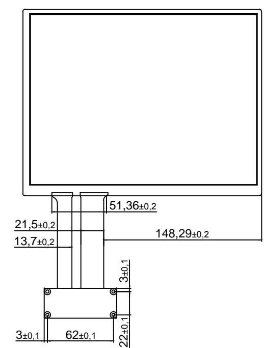
REAR VIEW
